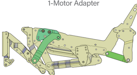
1-Motor Adapter
